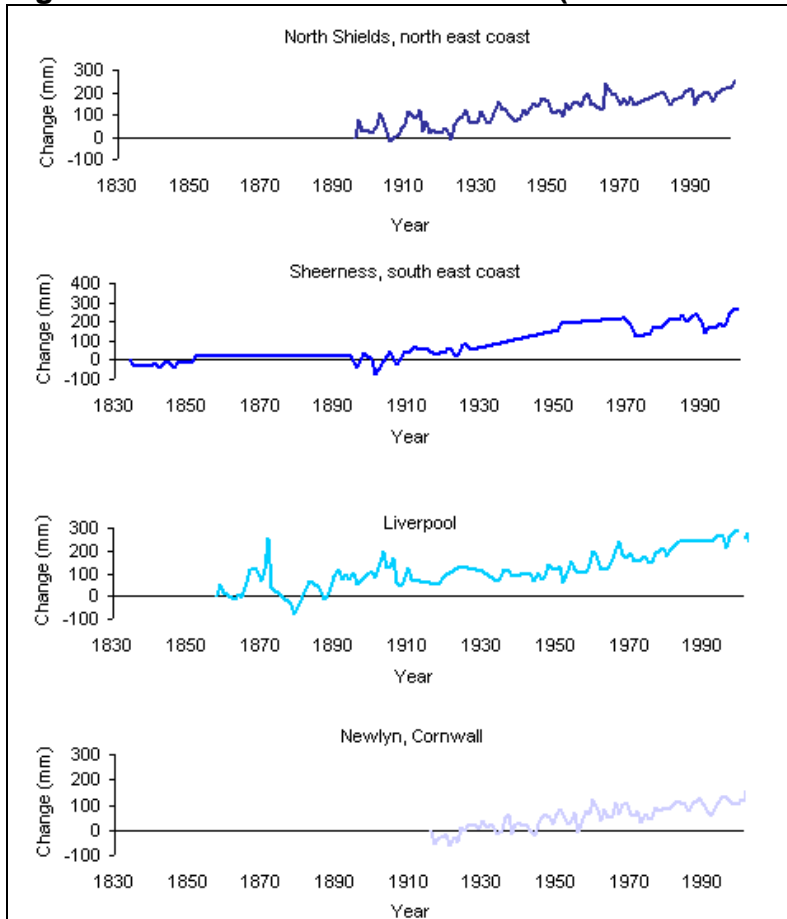
Figure 2-6 Recorded Sea Level Rise (Proudman Oceanographic Laboratory)
